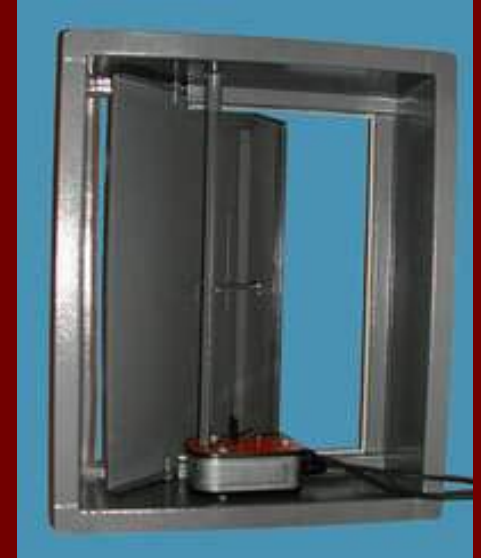
Smoke exhaust fan KDF-1 with falling shutter
